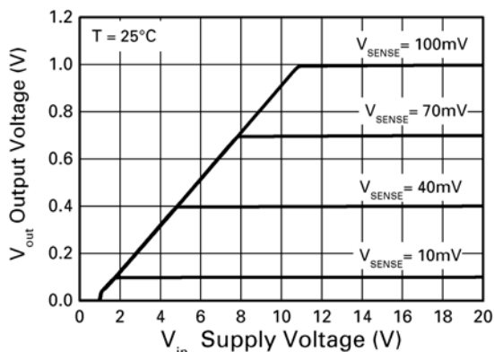
Transfer Characteristic
